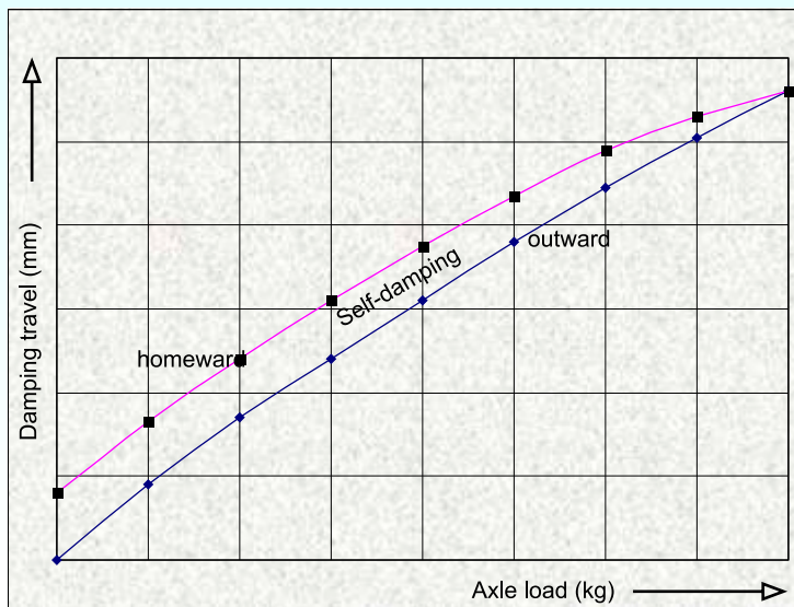
Suspension diagram
