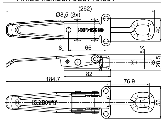
Spring latch L=31mm with plastic handle zinc plated Article number: 6S5716.001
