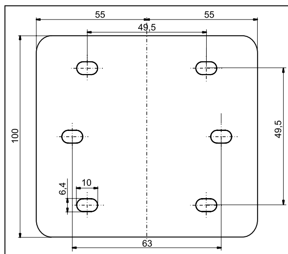
hole pattern
