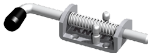
Spring latch L=31mm with plastic handle zinc plated Article number: 6S5716.001
