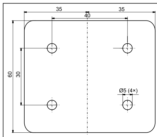
hole pattern
