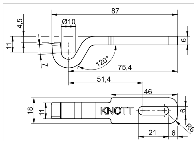
Engaging hook A11 straight, zinc plated Article number: 6S5752.001
