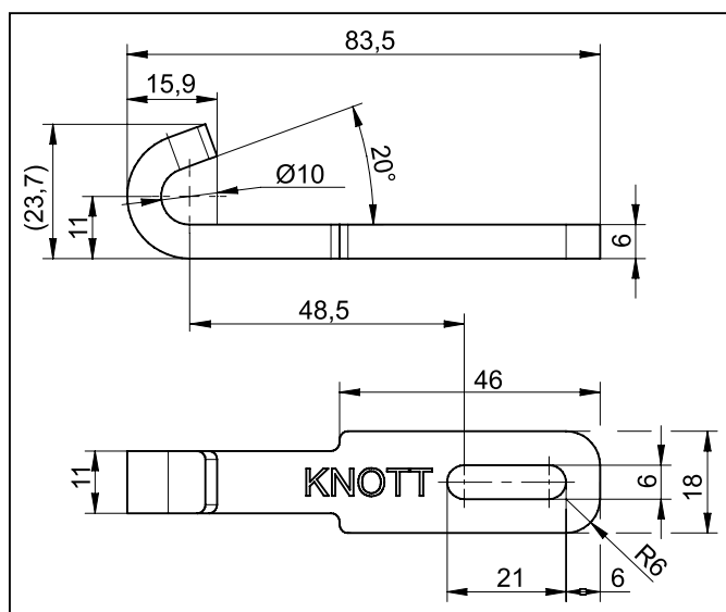
Adjustable overcentre latch FVS15 with spring, zinc plated Article number: 6S5684.001
