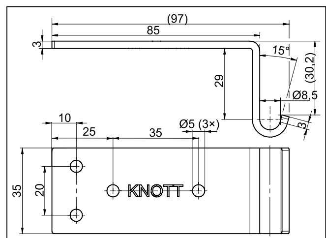
Catch plate C30 straight, zinc plated Article number: 6S5751.001
